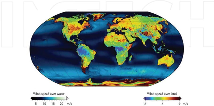
Figure 4. Worldwide average wind speed map, created based on wind speed measurements at the height of 80 m [94].
