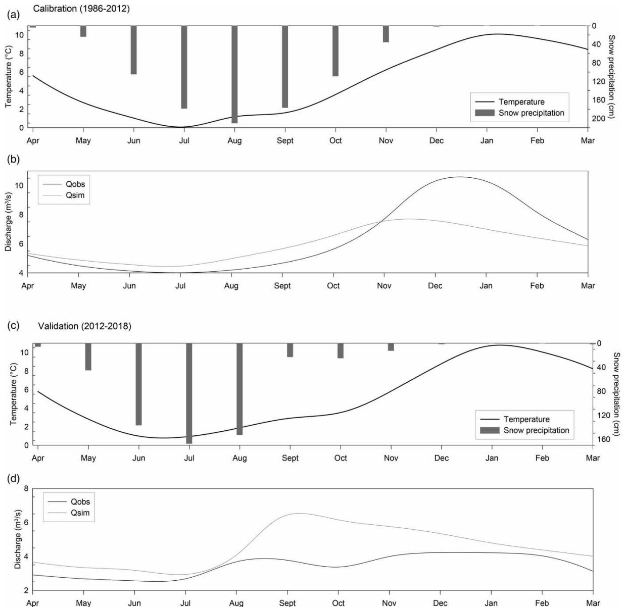
Figure 4 | Data and modelled results of precipitation, temperature and discharge averaged over the hydrological year for the calibration and validation model runs: (a and b) datasets are based on the calibration period for the Turbio River sub-basin; (c and d) datasets correspond to the validation time periods for the Turbio River sub-basin.
