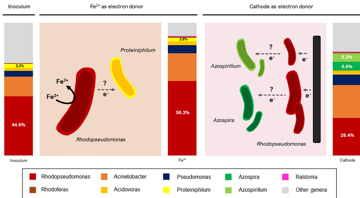
FIGURE 6 Microbial community analysis and schematic of the genus that might coexist depending on the electron donor. Stacked bars correspond to relative abundance at genus level of inoculum, ferrous iron as electron donor ( Fe^{2+} ) and cathode as electron donor (cathode). Left to the bars ( Fe^{2+} and cathode) the main genus and their possible interaction for each electron donor are represented.
