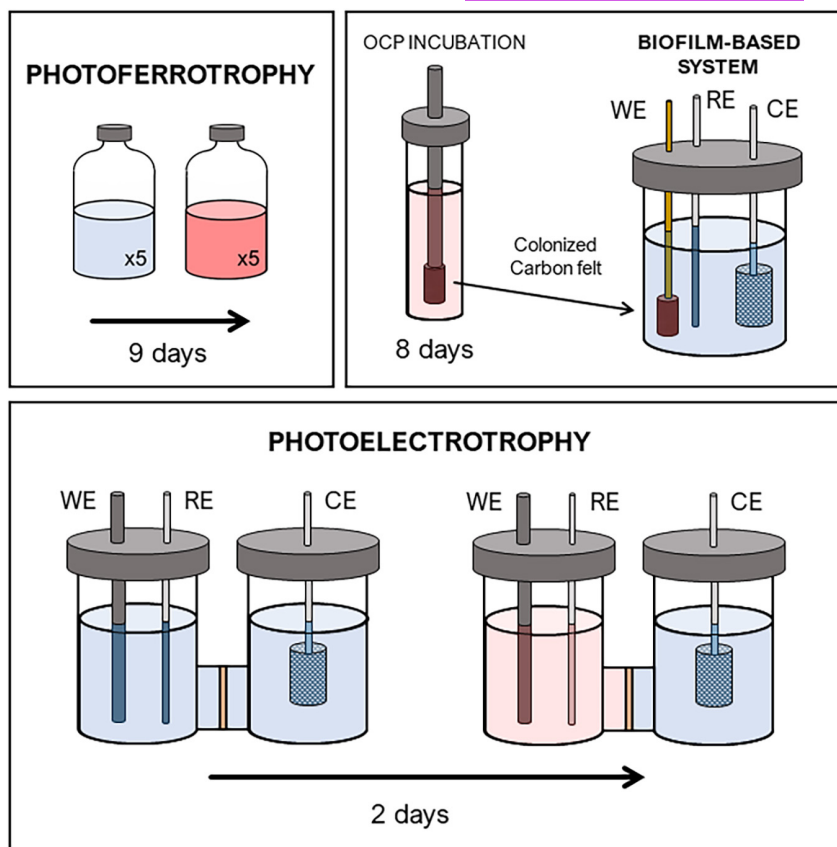
FIGURE 1 Schematic of the experiment set-up. Top left: Photoferrotrophy cultivation experiment. Top right: Biofilm-based experiment to assess electroactivity of the consortium.
